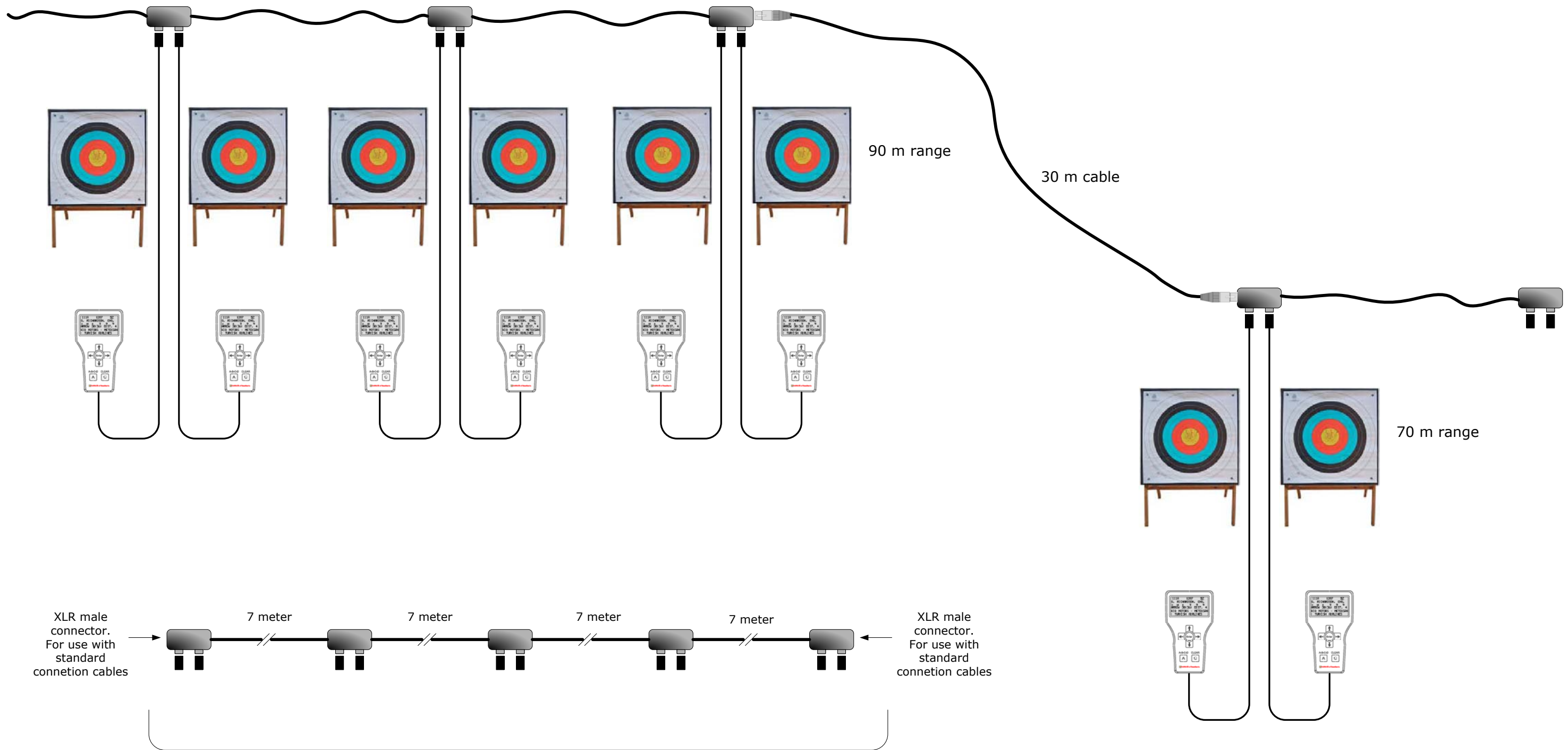
Score terminal connection cable. Each cable will handle 10 score terminals. Use standard Damage connection cables to extend.
